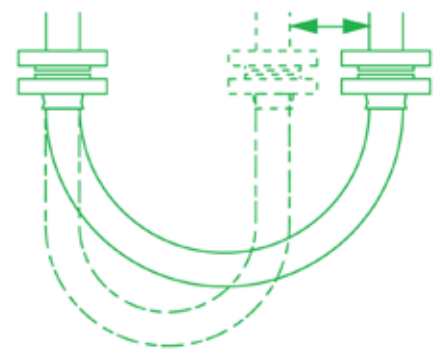
CORRECT - No flex at End Fittings
